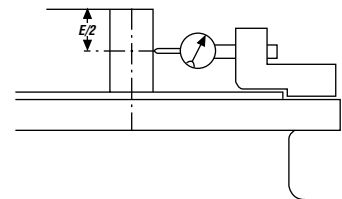
① Eccentricity of shaft in flanged motors
